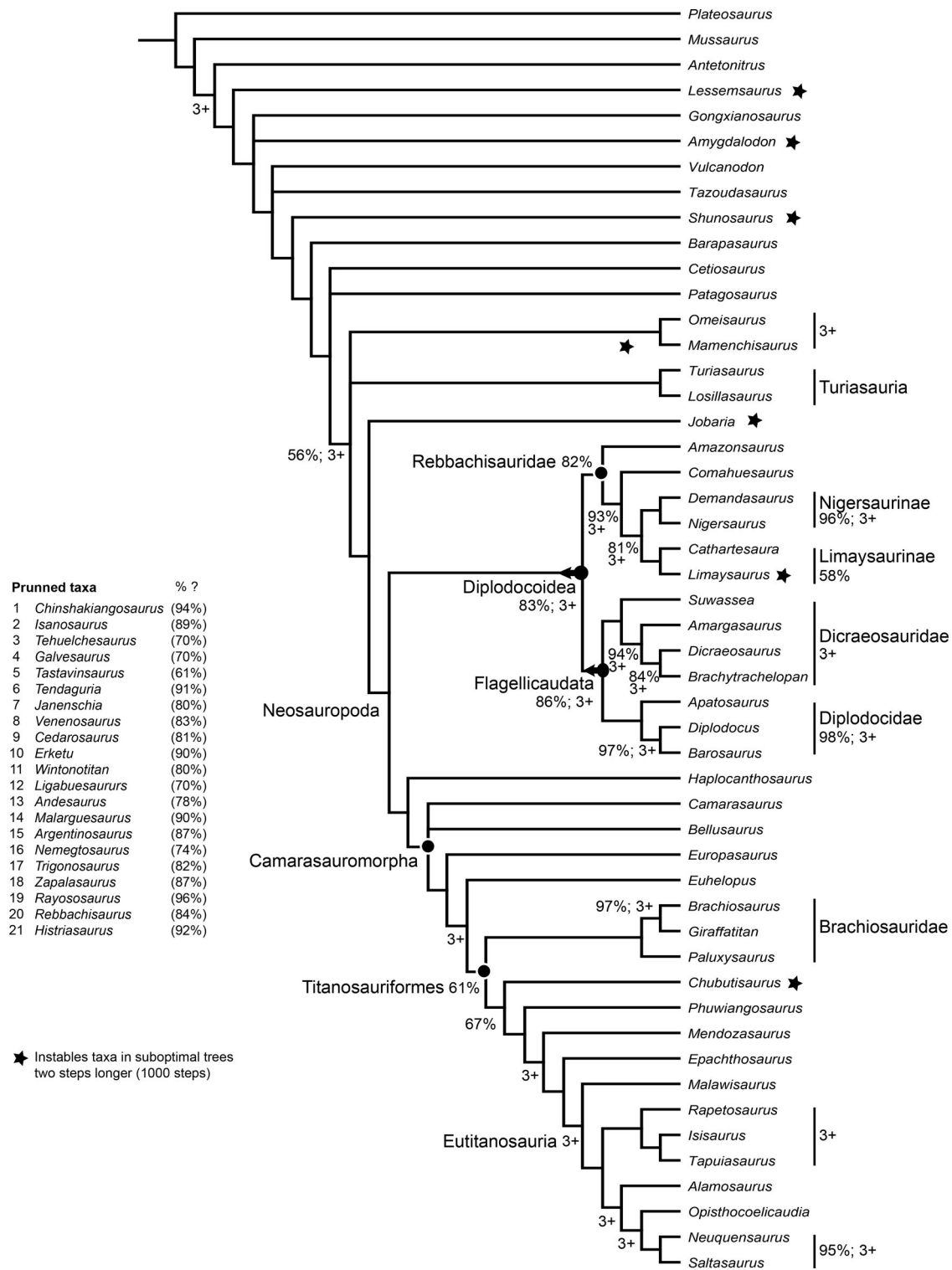
Figure 30. Strict consensus tree obtained after the pruning of more unstable taxa in suboptimal trees of one (left column) and two (star) steps longer than the MPT.
